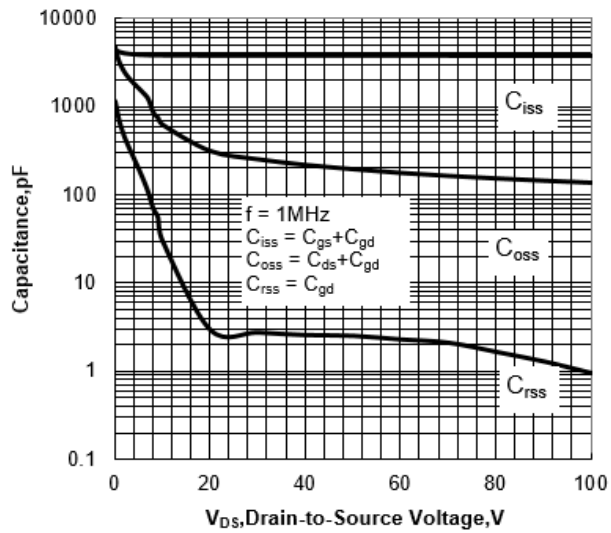
Figure 10 Capacitance Characteristics
